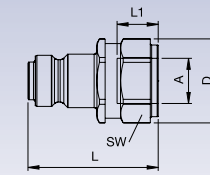
Female Thread
